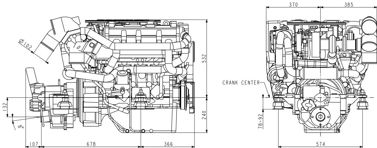
4LV195 with KMH50A marine gear
